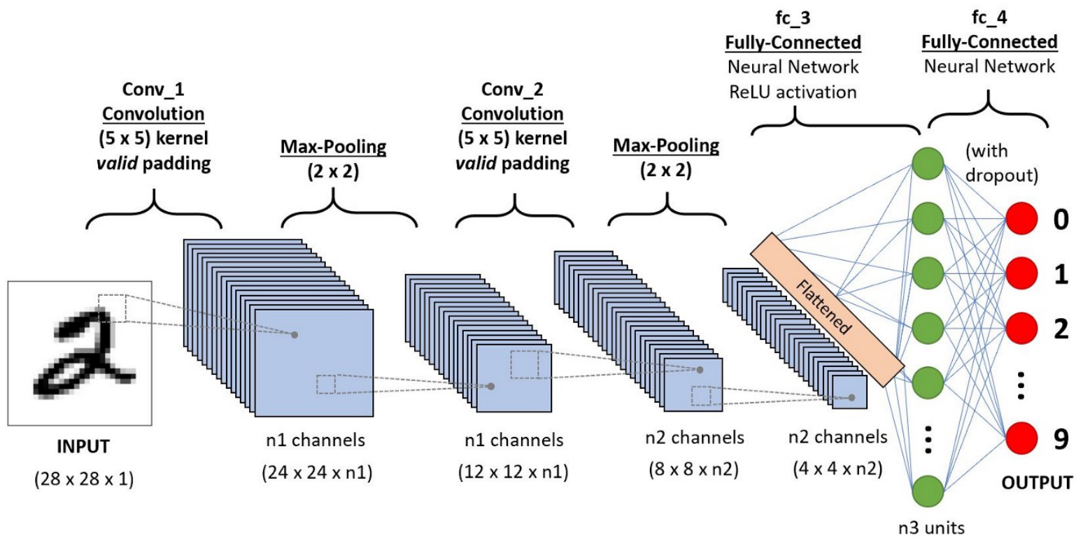
A CNN sequence to classify handwritten digits
